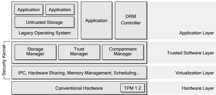
Fig. 2. Security architecture
