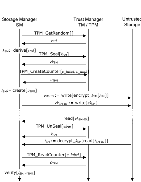
Fig. 5. SM initialization
