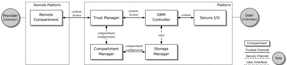
Fig. 1. System architecture
