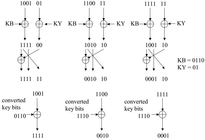
Fig. 4. Forming S_{rnd_q}
