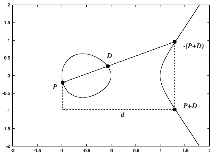
Fig. 1. Elliptic curve point addition differential over \mathbb{R}
