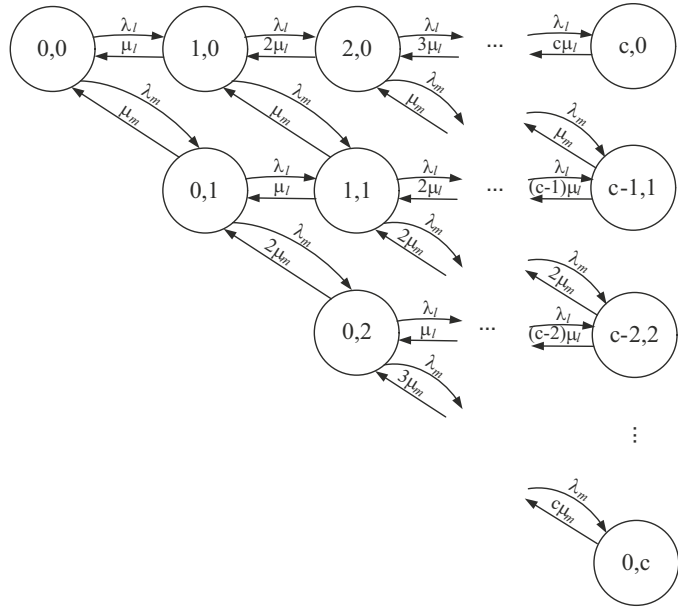
Fig. 6. Triangular DoS Markov chain model
